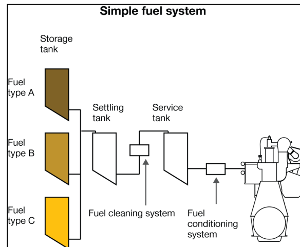
Figure 40 Schematic: Simple fuel system.
