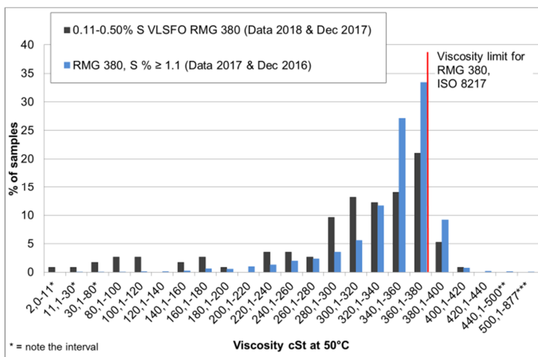
Figure 12 Viscosity distribution of fuels supplied as RMG 380. Blue bars: RMG 380 (equal or above 1.1% S). Black bars: RMG 380 (0.11 to 0.50% S). Data: LR FOBAS. Interpretation and evaluation: MAN ES.
