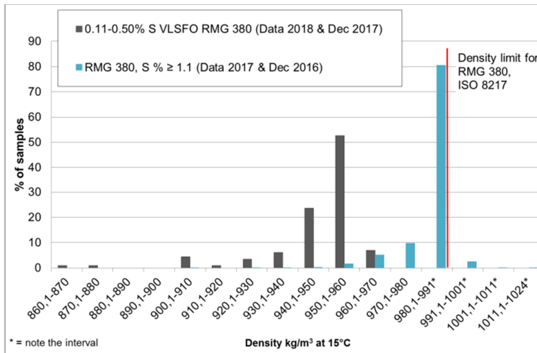
Figure 13 Density distribution of fuels supplied as RMG 380. Blue bars: RMG 380 (equal or above 1.1% S). Black bars: RMG 380 (0.11 to 0.50% S). Data: LR FOBAS. Interpretation and evaluation: MAN ES.
