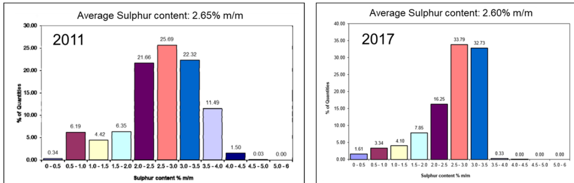
Figure 4 IMO Sulphur monitoring programme for residual fuels. In 2011, where the global limit for sulphur in the fuel was 4.50% S, 13% of the fuels were delivered with sulphur content higher than 3.50%. Note that the average sulphur content has not changed from 2011, it remains approx. 2.6% S.
