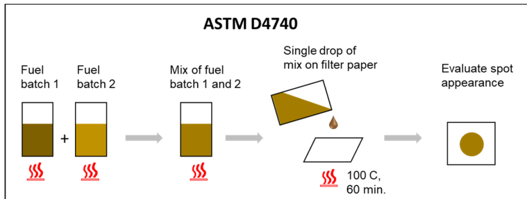
Figure 36 Compatibility testing of two different fuel batches. Schematic process flow: ASTM D4740.
