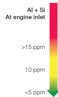
Figure 29 Recommended max. content of cat fines entering the engine. SL2017-638.
