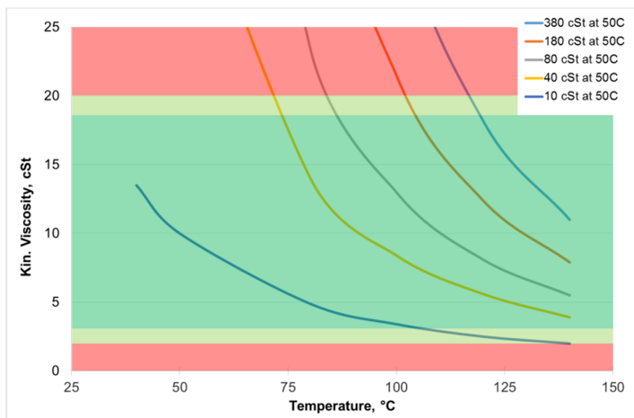
Figure 17 Temperature-viscosity relationship for fuels with different viscosity at engine inlet.
