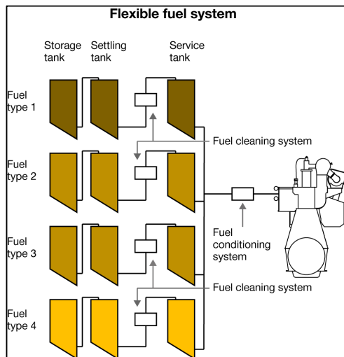
Figure 39 Schematic: Flexible fuel system.
