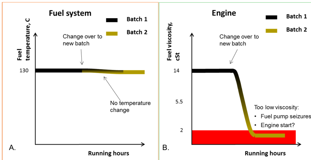
Figure 22 The figures show a change-over from a fuel with a viscosity of 380 cSt at 50°C (Batch 1) to a fuel with viscosity 8 cSt at 50°C (Batch 2) without changing the temperature of the fuel. Note that the viscosity at engine inlet will be too low.
