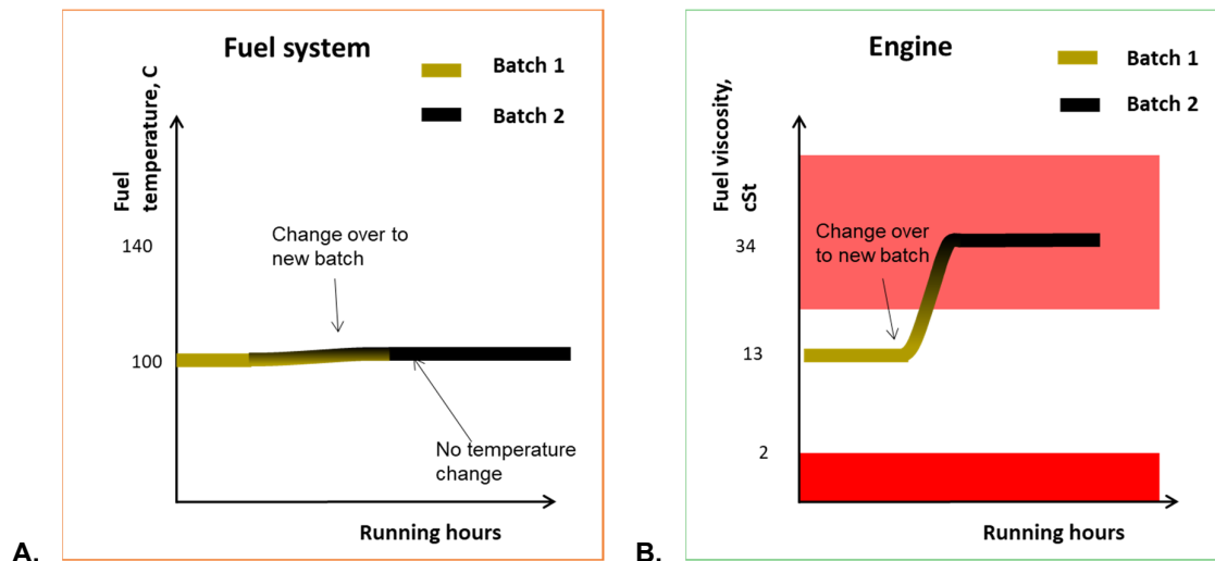
Figure 21 The figures show a change-over from a fuel with a viscosity of 80 cSt at 50°C (Batch 1) to a fuel with viscosity 380 cSt at 50°C (Batch 2) without changing the temperature of the fuel. Note that the viscosity at engine inlet will be too high.
