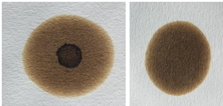
Figure 37 Spot test: photos of mixture of two different fuels on filter paper. A. Incompatible fuel blend. The black ring is the asphaltenes which have precipitated. B. Compatible fuel blend. ASTM D4740 shows 5 different classes for compatibility, ranging from compatible to incompatible.
