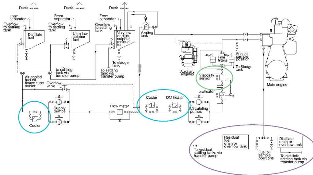
Figure 20 Fuel System diagram. Blue circles: coolers. Green circle: viscosimeter / viscosity sensor.
