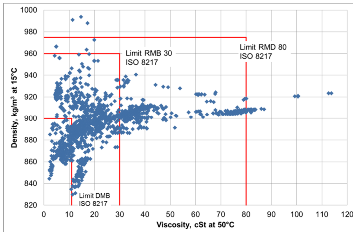
Figure 9 Density, kg/m 3 at 15°C and viscosity, cSt at 50°C of 0.10% S ULSFO-RM supplied in 2015-2016. Data: LR FOBAS. Interpretation and evaluation: MAN ES.
