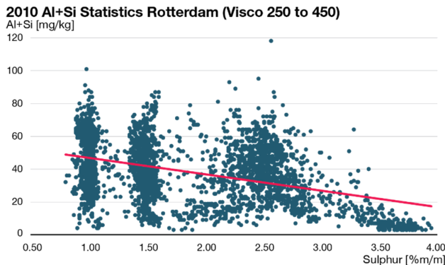
Figure 30 Cat fines content in relation to sulphur content in the fuel as bunkered. Data from 2010 showing both SECA limits of max. 1.5%S and 1.0%S. Data courtesy: VPS, evaluation: MAN ES.
