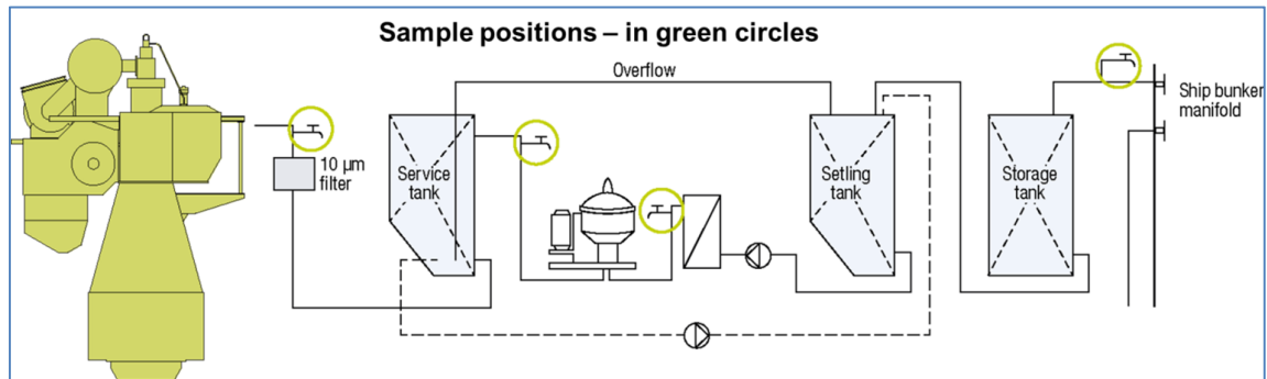
Figure 47 Examples of fuel sampling positions.
