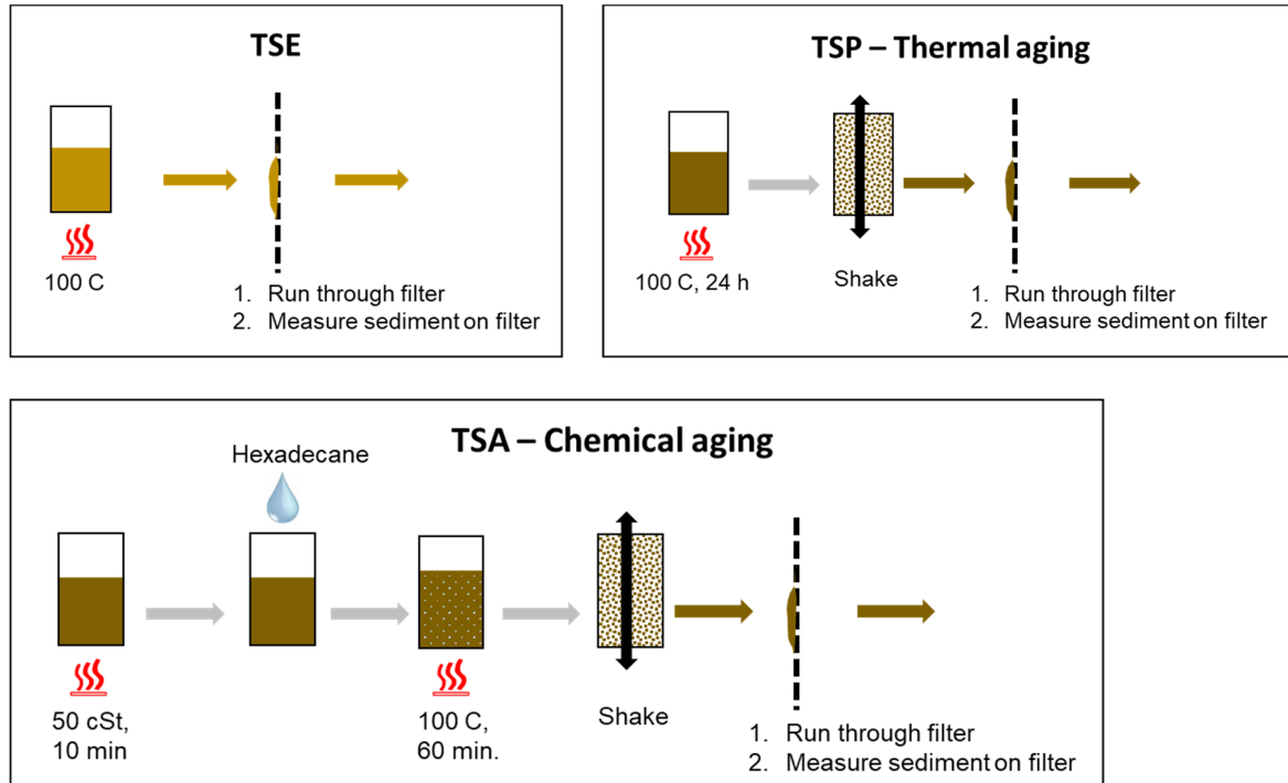
Figure 35 Fuel stability testing. For DM-types: TSE (ISO 10307-1). For RM-types: TSP and TSA (ISO 10307-2)
