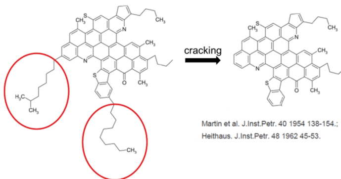
Figure 15 Cracking changes the asphaltenes.
