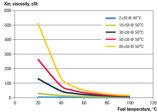
Figure 19 Temperature–viscosity relationship for low-medium viscosity fuels.
