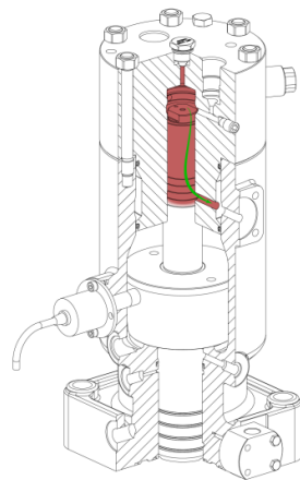
Figure 23 ME engine - Fuel Oil Pressure Booster. Usually no problem with low-viscosity fuels because: 1. Plunger velocity is governed by supply pressure. 2. At start conditions it has 75-78% of full load supply pressure. 3. Long leakage path (green).
