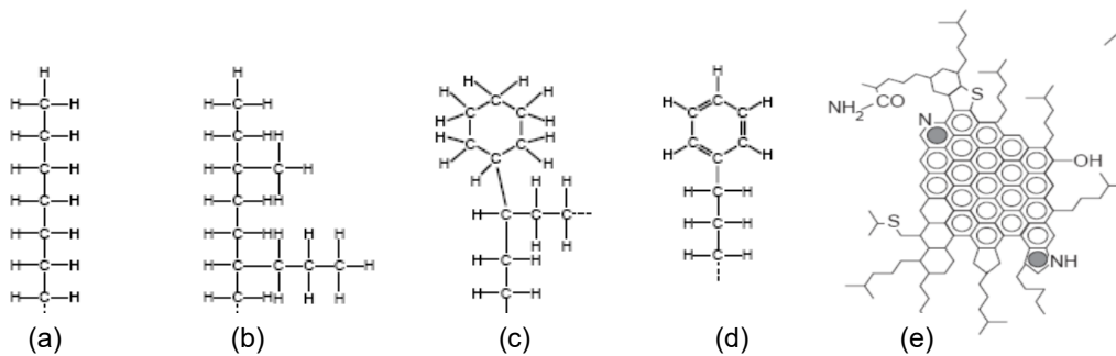
Figure 14 Schematic pictures of (a + b) Paraffins, (c) Naphtenes (d) Aromatics and (e) Asphaltene.
