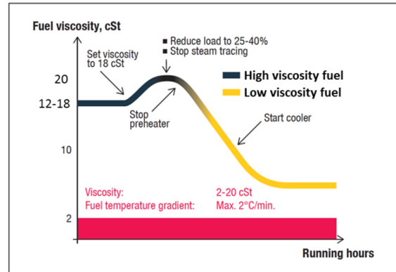
Figure 26 Change-over procedure from warm, high viscosity fuel to cold, low viscosity fuel.
