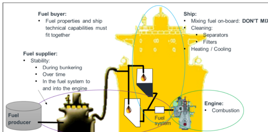
Figure 5 Purchasing fuel. Responsibilities and actions
