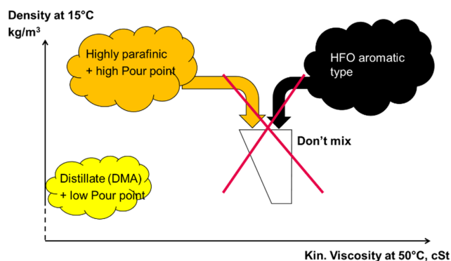
Figure 38 Keep different fuels separated.
