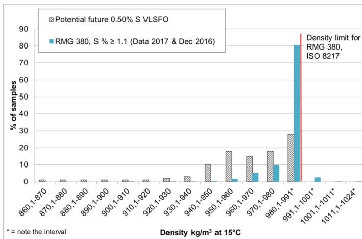
Figure 27 Density distribution for RMG 380. Blue bars: data from 2017. Striped bars: Expected/potential density distribution for 0.50%S VLSFO. Data courtesy: LR FOBAS, evaluation and interpretation: MAN ES.
