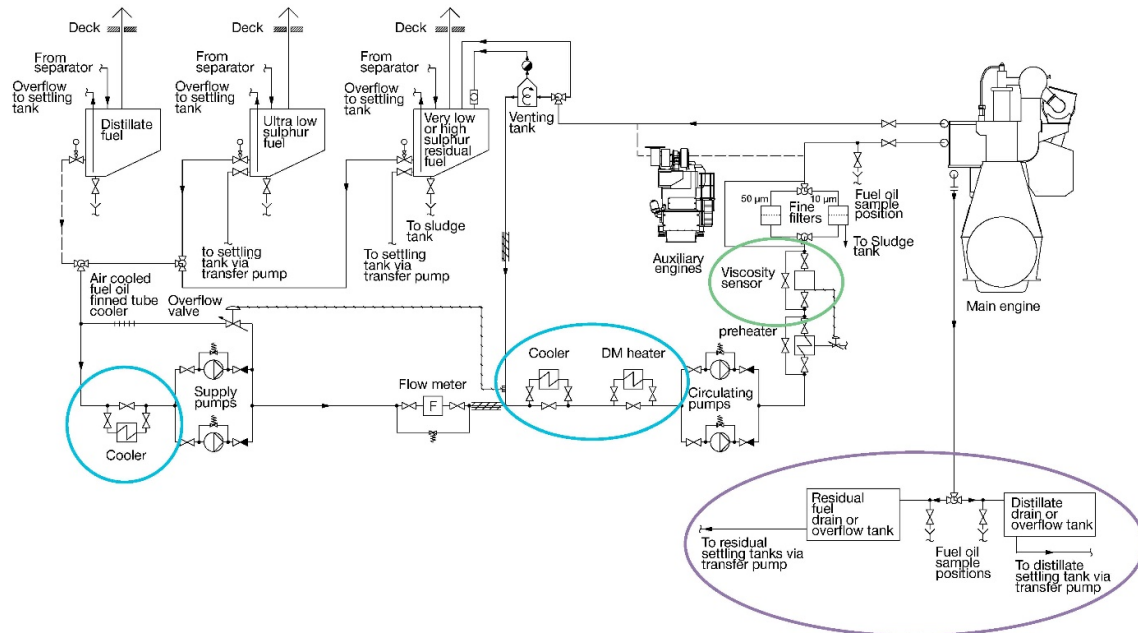
Figure 45 Fuel system diagram. Purple circle: fuel pump drain arrangement.
