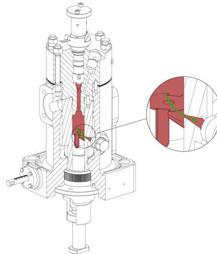
Figure 24 MC engine - cam driven Fuel Oil Injection Pump. Test to find the low-viscosity limit because: 1. Plunger velocity is governed by engine rpm. 2. At start conditions it has 15% of the full load engine rpm. 3. Short leakage path (green). Solution: Use unworn fuel pumps.
