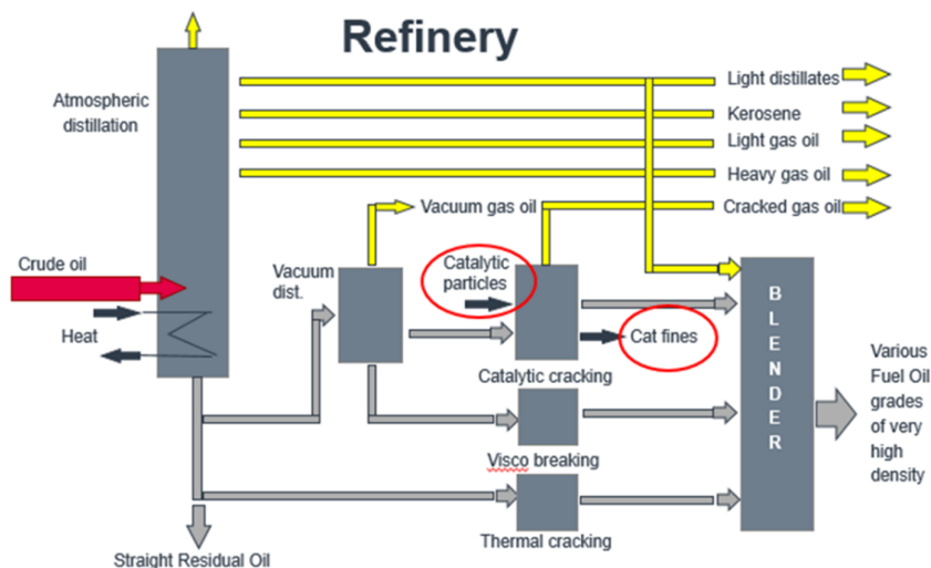
Figure 11 Simplified schematic figure of a refinery.
