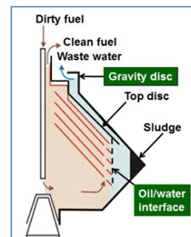
Figure 28 Schematic of bowl in classic separator. Courtesy: Alfa Laval
