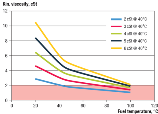
Figure 18 Temperature–viscosity relationship for very low viscosity fuels.
