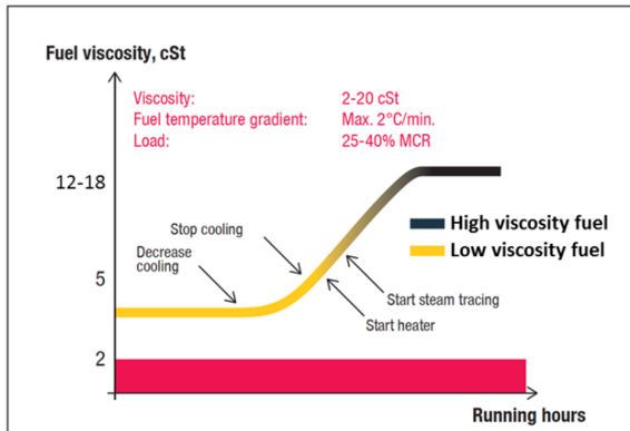
Figure 25 Change-over procedure from cold, low viscosity fuel to warm, high viscosity fuel.
