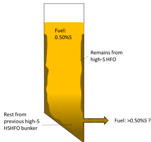
Figure 42 Fuel tank filled with 0.50% S VLSFO on top of HSHFO. The rest may be high in sulphur. The rest is mixed in the new batch and may cause increased sulphur content in the fuel leaving the tank.
