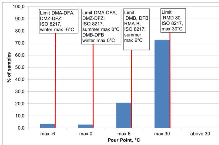
Figure 10 Distribution of pour points of 0.10% S ULSFO-RM supplied in 2015-2016. Data: LR FOBAS. Interpretation and evaluation: MAN ES.
