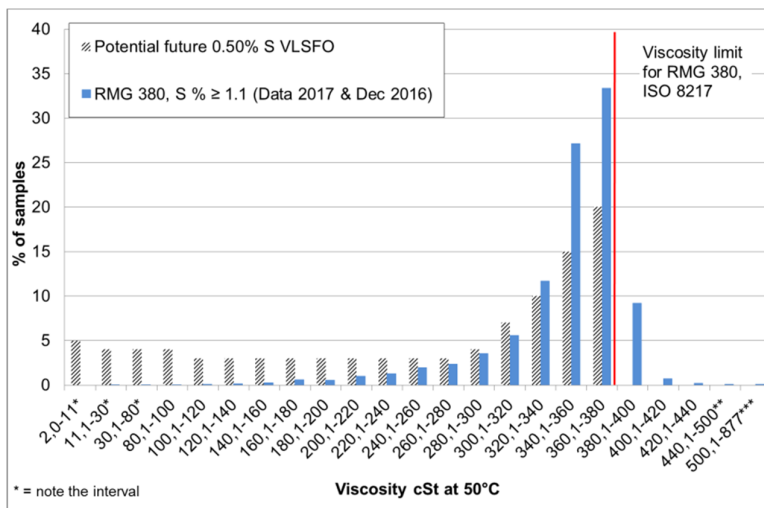
Figure 16 Viscosity distribution for RMG 380. Blue bars: Data from 2017. Striped bars: Expected/potential viscosity distribution for 0.50% S VLSFO. Data: LR FOBAS. Interpretation & evaluation: MAN ES.
